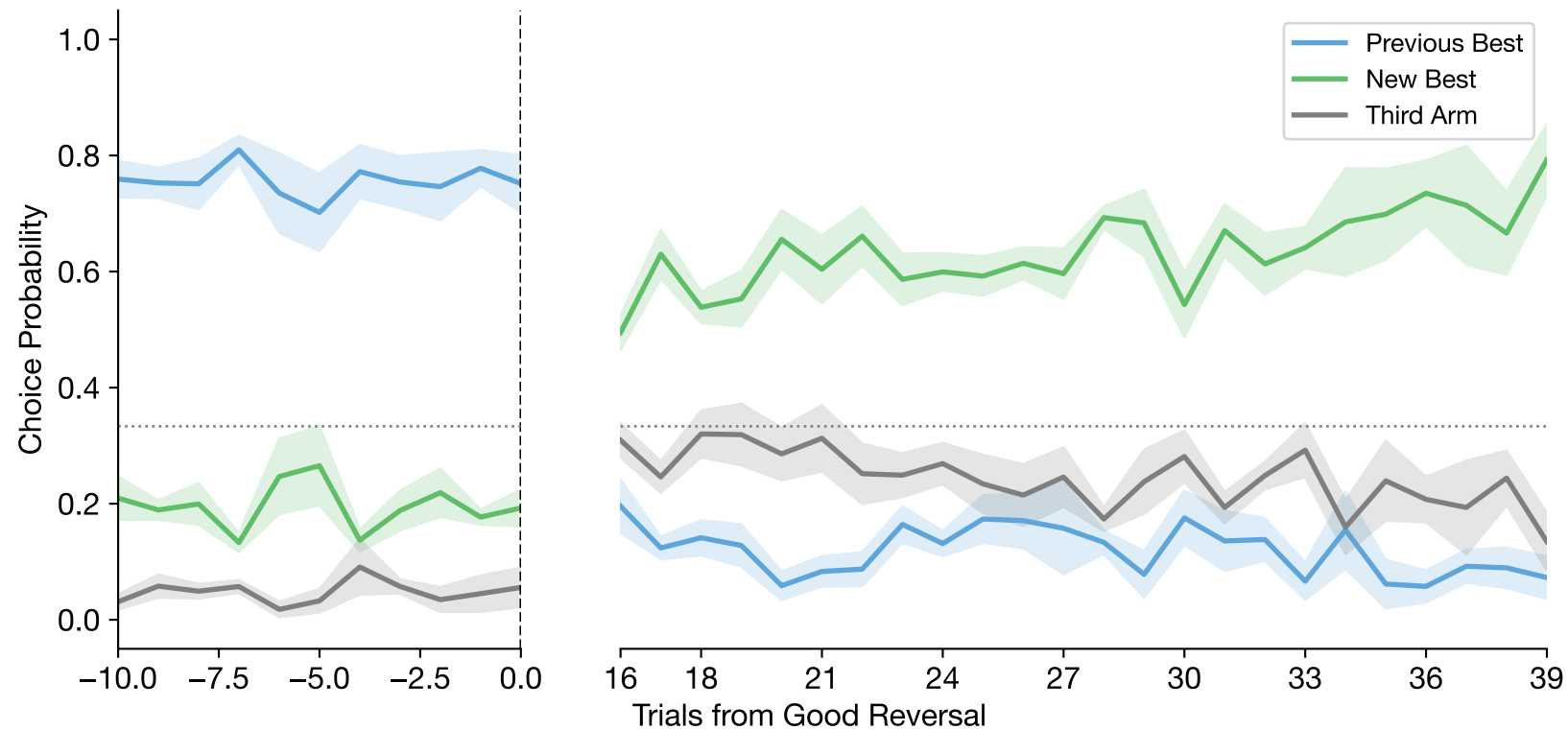
Good Reversal-Aligned Choices (mean \pm se across subjects | n=6 subjects, n=192 reversals) (Skipping first 15 trials post-reversal)
